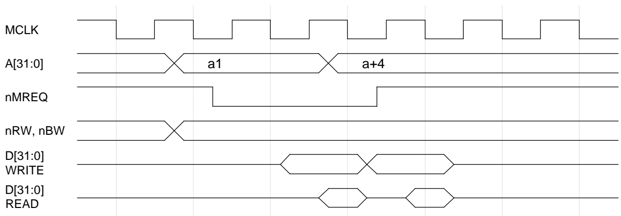
Figure 44: Two Word Sequential Read or Write
