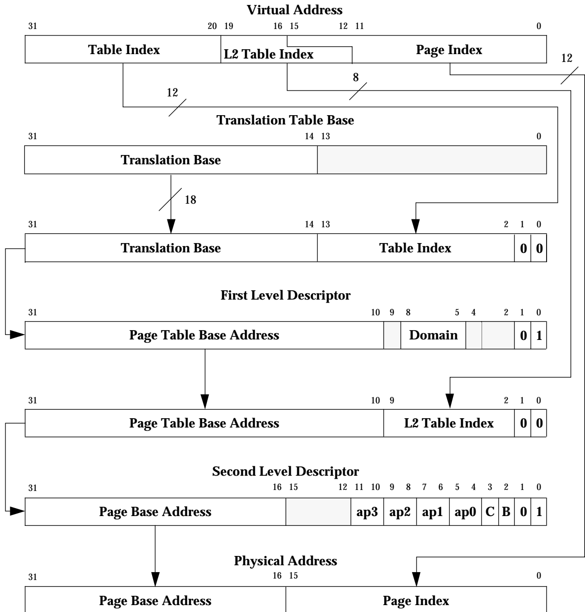
Figure 40: Large Page Translation
