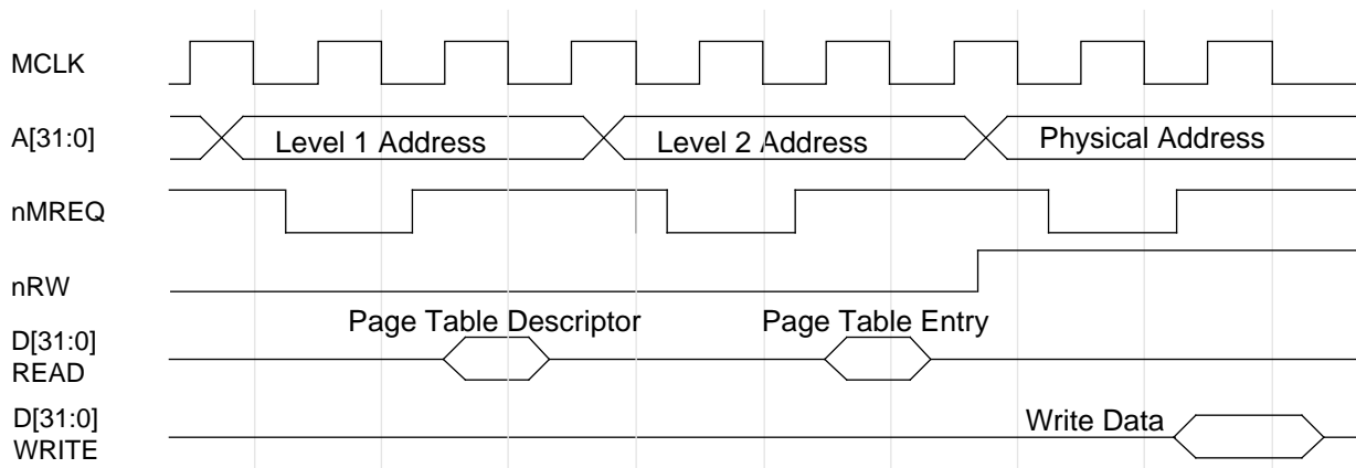
Figure 48: Translation Table-walking Sequence (write) For Page
