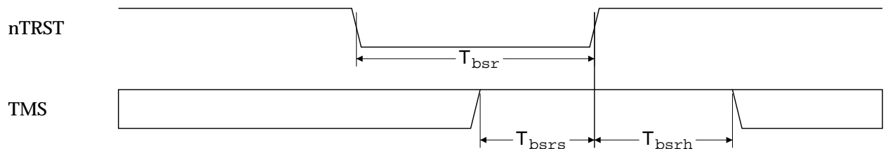
Figure 56: Boundary Scan Reset Timing
