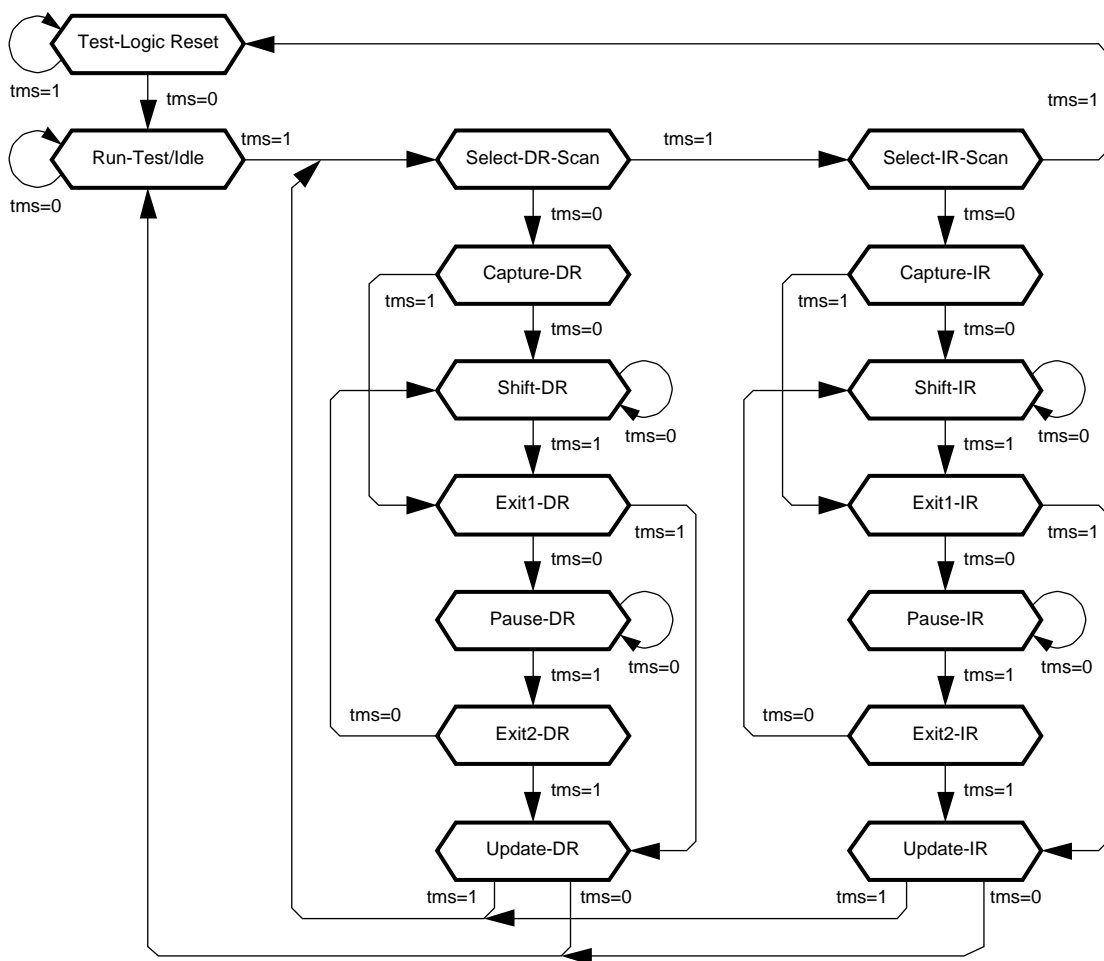
Figure 52: Test Access Port (TAP) Controller State Transitions
