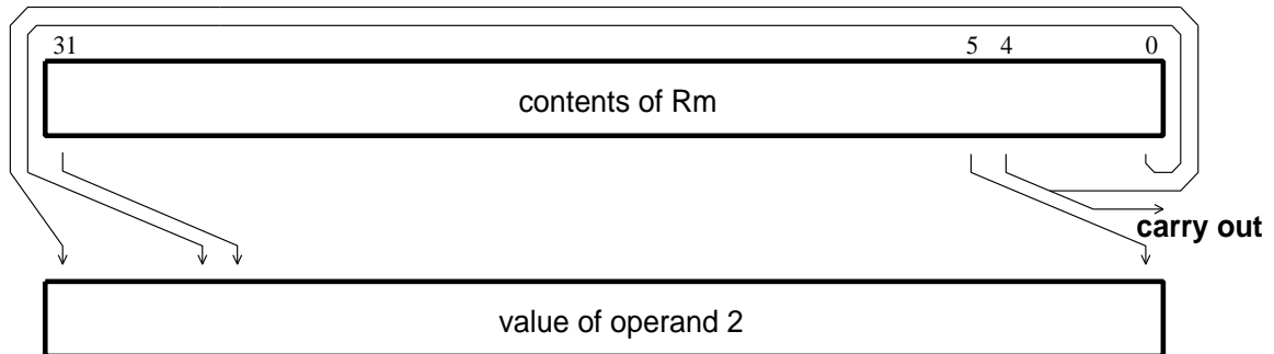
Figure 15: Rotate Right
