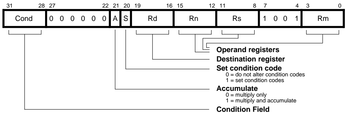
Figure 18: Multiply Instructions
